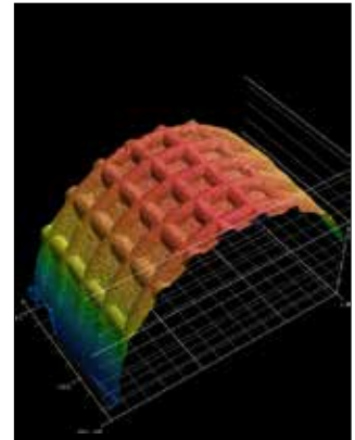
Macro-/microstructure on shaft of slip-cast implant made of ATZ.
