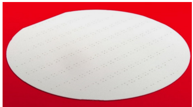
Polished LTCC wafer with Au vias for anodic bonding with silicon MEMS wafer.
