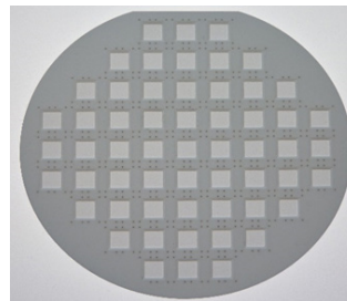
Bondable LTCC wafer with integrated cavities for ASIC packaging.
