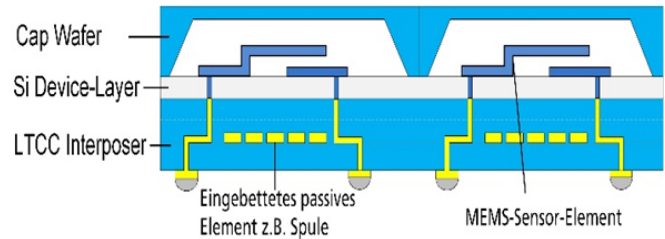
Schematic diagram of wafer-level packaging of LTCC wafer with silicon MEMS wafer.
