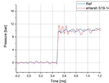
Characteristic curves of the pressure sensors under dynamic pressure change (shock tube measurement).
