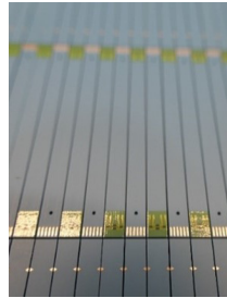
Ceramic multilayer sensor element in multiple panel manufacturing.
