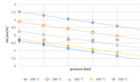
Characteristic curves of pressure sensors in the temperature range of 100–500 °C.
