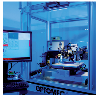
Deposition of functional layer by aerosol printing.
