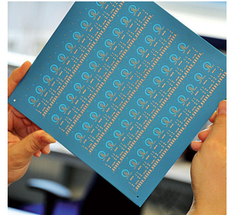
LTCC based pressure sensors (8" x 8").
