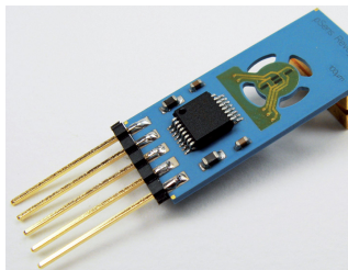
LTCC-based pressure sensor.
