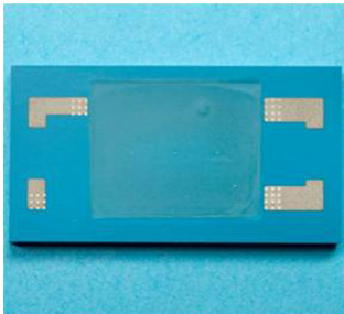
100 W high-power transformer in LTCC with monolithic integrated ferrite plates.
