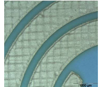
Enlarged picture of a coil section after stencil printing.
