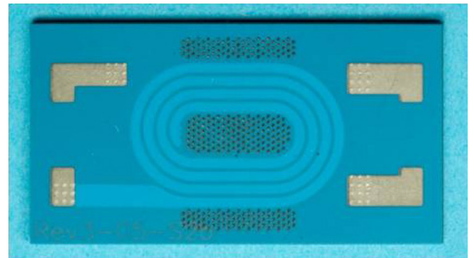
100 W high-power transformer with ferritic vias (volume = 0.8 cm 3 ).
