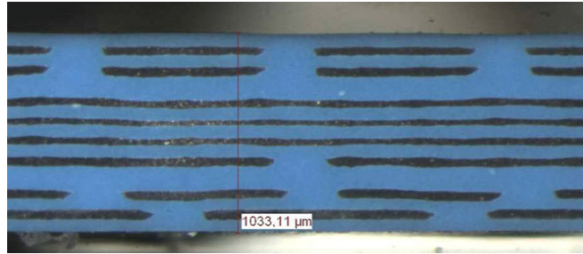
Cross section of a sintered LTCC transformer with a silver-layer thickness of 50 μm and eight metallization layers.
