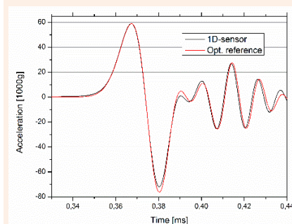
Acceleration measurement 3D LTCC package up to 100 000 g (courtesy: Fraunhofer EMI)
