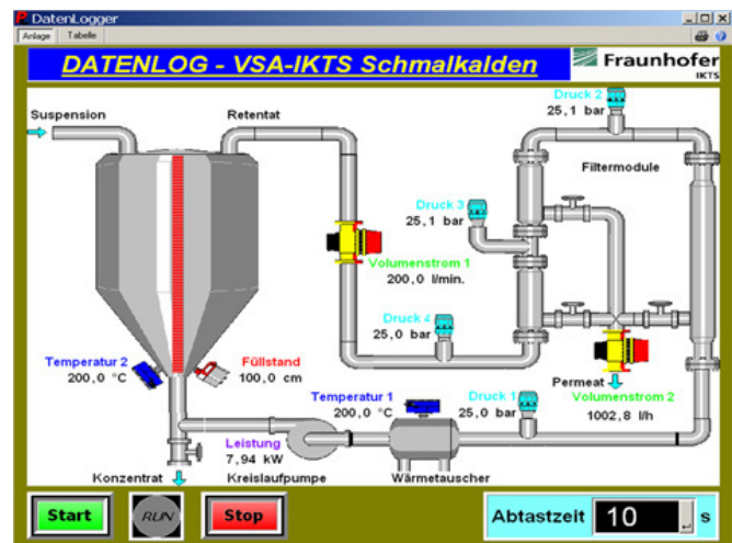
Flow sheet of membrane plant.
